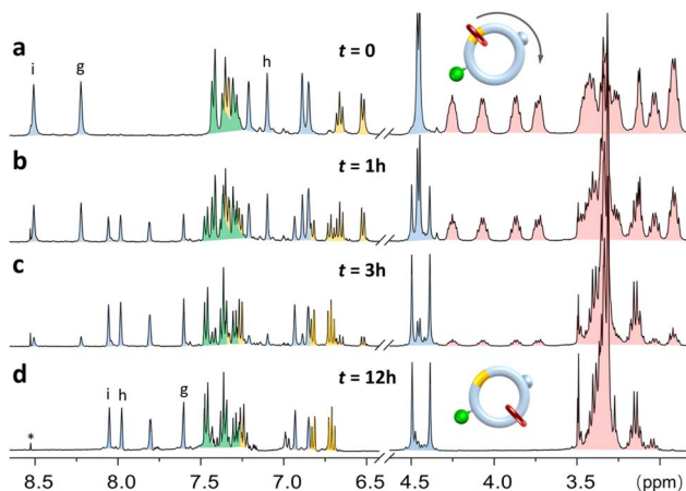
Fig. 7 Partial 1 H NMR (400 MHz, 298 K, \text{DMSO-d}_6 ) spectra of [\text{I-BnM}]^- heated at 338 K for (a) 0 h; (b) 1 h; (c) 3 h; and (d) 12 h * Impurity.
