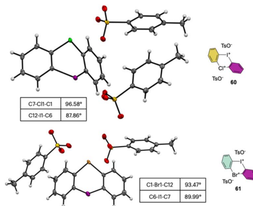
Fig. 9 X-ray structures of 60 and 61.
