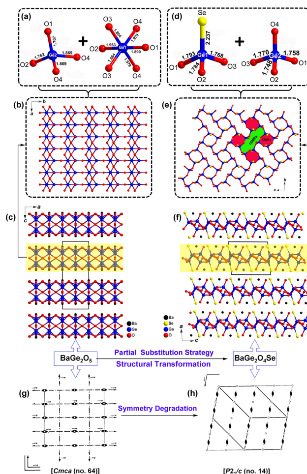
Fig. 1 Structural transformation from oxide \text{BaGe}_2\text{O}_5 to oxychalcogenide \text{BaGe}_2\text{O}_4\text{Se} : (a and d) coordination environment of [\text{GeO}_4] , [\text{GeO}_3\text{Se}] , and [\text{Ge}_2\text{O}_4] units with the atom numbers outlined; (b and e) 2D [\text{Ge}_2\text{O}_5]^{2-} and [\text{Ge}_2\text{O}_4\text{Se}]^{2-} anion layers; (c and f) the 2D layered structures viewed from the b direction; (g and h) symmetry degradation from Cmca (no. 64) to P2 1 /c (no. 14).
