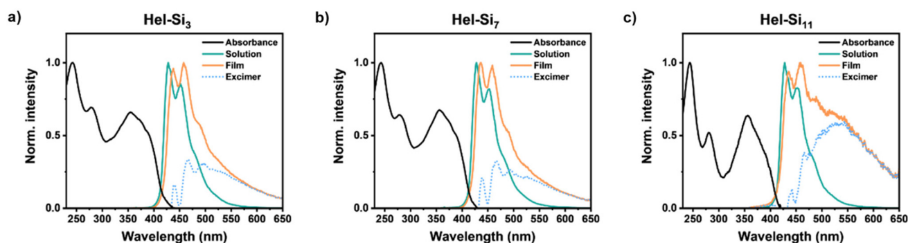
Fig. 5 Absorption and emission spectra of M - Hel-Si n (a, b, and c for n = 3, 7 and 11 , respectively) in 10 -5 M THF solution and in the solid state recorded as a thin film. The dotted blue trace is the difference between the emission spectra in the solid state and solution to show the excimer. The spectra have all been normalized to unit intensity. The spectra for P enantiomers are similar (Fig. S70†).
