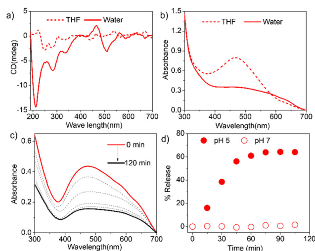
Fig. 3 (a) CD and (b) UV/vis spectra of P1S in water and THF. (c) Time-dependent UV/vis spectra of P1S at pH 5 buffer solution. Each spectrum was taken at 15 min time intervals. (d) %release of NMIS from aqueous solution of P1S solution at pH 5 or pH 7 buffer (concentration of P1S = 1.0 mg mL -1 ).
