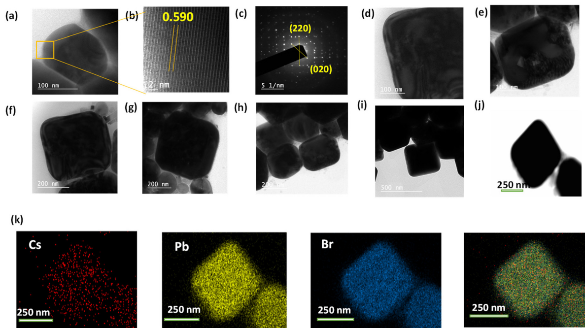
Fig. 3 TEM images of \text{CsPb}_2\text{Br}_5 (a) at 100 nm, (b) fringes at 2 nm, (c) SAED pattern, (d and e) images at 100 nm, (f–h) images at 200 nm, (i) image at 500 nm, and (j and k) elemental mapping of the microcrystal.
