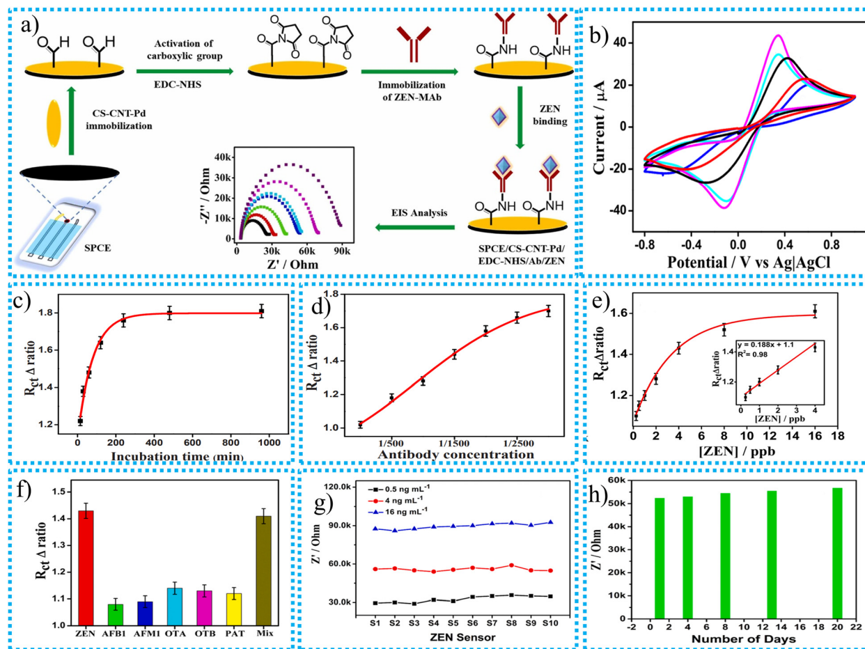
Fig. 12 (a) The CNT-based CSCNT-Pd-based immunosensor synthesis procedure, (b) CV curves for the impact of modification on the SPCE electrode, (c) electrochemical impedimetric responses ( \Delta \text{ratio} ) of the SPCE/CS-CNT-Pd/ZEN-MAb modified electrode after incubation with 4 ng mL -1 of ZEN at different incubation time intervals, (d) impedimetric responses of the SPCE/CS-CNT-Pd/ZEN-MAb modified electrode to varying concentrations of antibody (ZEN-MAb), (e) the calibration curve of the ZEN immunosensor based on the change in R_{ct} , (f) electrochemical impedimetric responses of the fabricated immunosensor, (g) impedance responses of ten independent immunosensor sets towards ZEN detection, (h) impedance responses of the ZEN immunosensor for 20 days under ambient conditions toward the detection of 2.0 ng mL -1 of ZEN. 174
