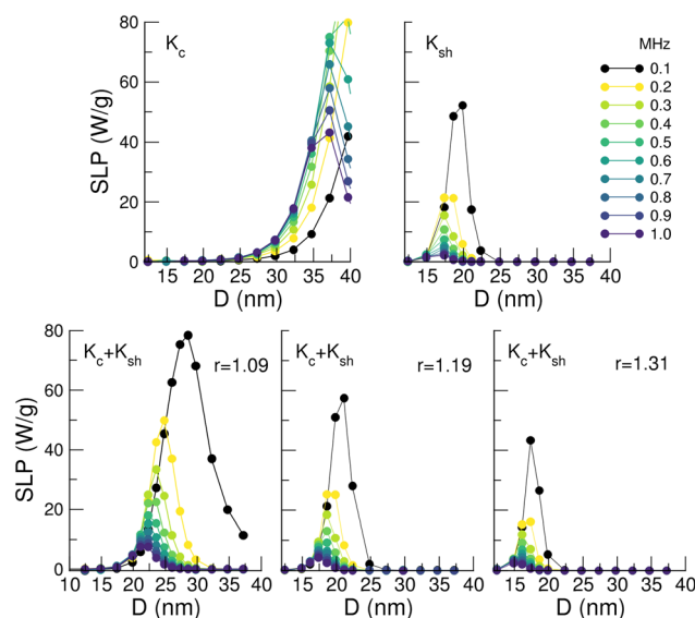
Fig. 7 Size-dependence of the SLP for different frequencies and maximum AC fields achieving the Brezovich criterion H_{\text{max}} \cdot f = 4.85 \times 10^8 \text{ A m}^{-1} \text{ s}^{-1} . Upper panels show the case for spherical particles with only crystalline cubic (left, K_c ) and only shape (right, with K_{\text{sh}} = K_c ) anisotropies, respectively. Lower panels correspond to ellipsoidal particles of aspect ratios r = 1.09, 1.19 , and 1.31 with uniaxial shape anisotropy added to the cubic one.
