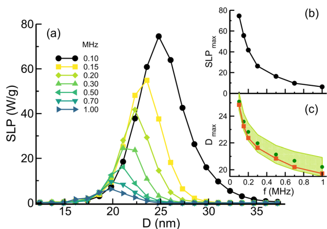
Fig. 6 (a) Dependence of the SLP on nanoparticle diameter D and aspect ratio r = 1.12 ( K_{\text{sh}} \approx 6.5 \text{ kJ m}^{-3} ) for the frequencies indicated in the legend, and AC fields respecting the Brezovich criterion. A cubic anisotropy constant equal to that of magnetite has been considered. (b) and (c) display the frequency dependence of the maximum value of SLP and the diameter at which D_{\text{max}} is obtained. In (c), the green circles indicate the D_{\text{max}} values obtained from eqn (3), using a value of f_0 = 10^9 \text{ Hz} and the green shaded region indicates the range obtained when varying f_0 between 0.5 and 1.5 \times 10^9 \text{ Hz} .
