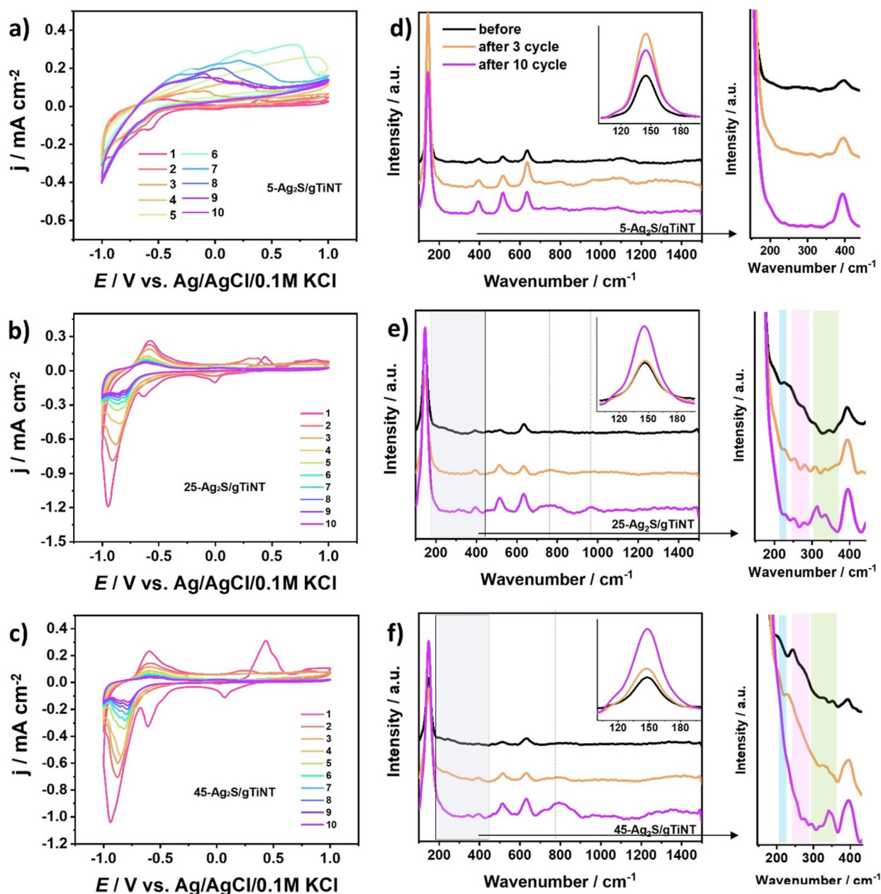
Fig. 7 Cyclic voltammograms of (a) 5- \text{Ag}_2\text{S/gTiNT} , (b) 25- \text{Ag}_2\text{S/gTiNT} , (c) 45- \text{Ag}_2\text{S/gTiNT} and Raman spectra before CVs and after 3 or 10 CVs cycles for (d) 5- \text{Ag}_2\text{S/gTiNT} , (e) 25- \text{Ag}_2\text{S/gTiNT} , (f) 45- \text{Ag}_2\text{S/gTiNT} in 0.5 M \text{Na}_2\text{SO}_4 electrolyte (scan rate 50 \text{ mV s}^{-1} ). All the graphs on the right are insets of the Raman graphs.
