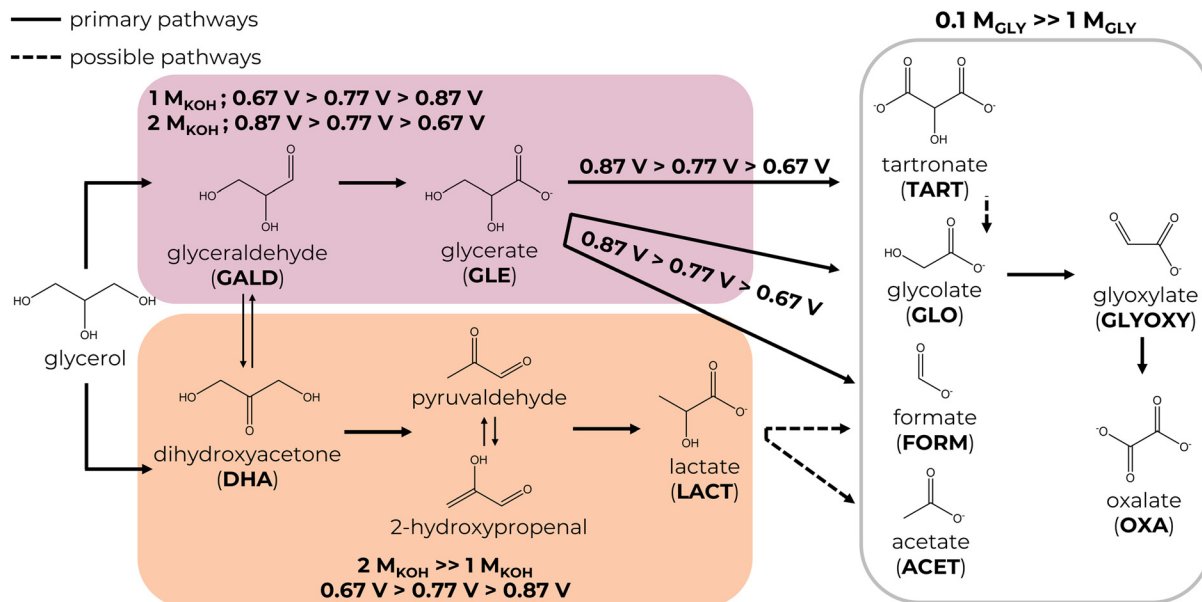
Scheme 2 Proposed GEOR mechanism on the \text{Pt}_{\text{NPs}}/\text{CFP} electrodes in an alkaline medium.
