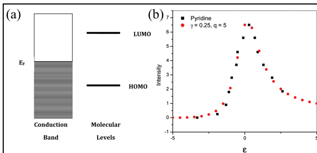
Fig. 2 (a) Energy levels of the metal–molecule system. (b) Fano profiles of the voltage-dependent profile of the 1008\text{ cm}^{-1} line of pyridine, wherein red circles represent simulated Raman line shape and black squares represent the experimental data. Reproduced from ref. 28 with permission from [American Chemical Society], copyright [2010].
