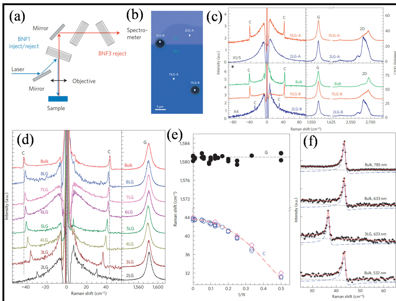
Fig. 7 (a) Schematic diagram of our single monochromator with three BraggGrate notch filters (BNF). (b) Optical micrograph of the FLG sample. 2LG-A/11LG-A and 2LG-B/11LG-B denote supported and suspended flakes, respectively, (c) S/AS spectra of supported flakes and suspended flakes, top and bottom, respectively, in the C peak region (left) and S spectra in the G/2D peaks region (right), (d) S/AS Raman spectra for the C peak spectral region (left) and S Raman spectra for the G peak spectral region (right). (e) Peak positions Pos(G) (filled black circles) and Pos(C) (open blue circles) as a function of inverse layer number, (f) C peaks with BWF fit for bulk graphite and 3LG. Fitted curve (solid red lines); background (dashed lines); BWF component (dash-dotted lines). Reproduced from ref. 45 with permission from [Springer Nature], copyright [2012].
