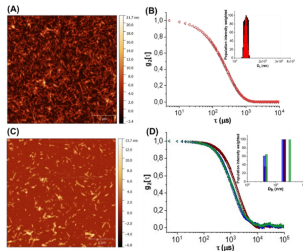
Fig. 2 (A) 5 \mu\text{m} \times 5 \mu\text{m} AFM image of the CNC* suspension in H 2 O dried on mica. (B) Autocorrelation functions of the CNC (black) and CNC* (red) dispersed in MilliQ water. Top right size populations overlay (weighted on the scattered light intensity contribution) obtained through Contin's fitting. (C) 5 \mu\text{m} \times 5 \mu\text{m} AFM image of the CNC*-Au-LA 4 suspension in H 2 O dried on mica. (D) Autocorrelation functions of CNC*-Au-LA 4 (brown), CNC*-Au-Glc 5 (blue), and CNC*-Au-Man 6 (green) dispersed in MilliQ water. Top right size populations overlay (weighted on the scattered light intensity contribution) obtained through double exponential fitting on autocorrelation functions.
