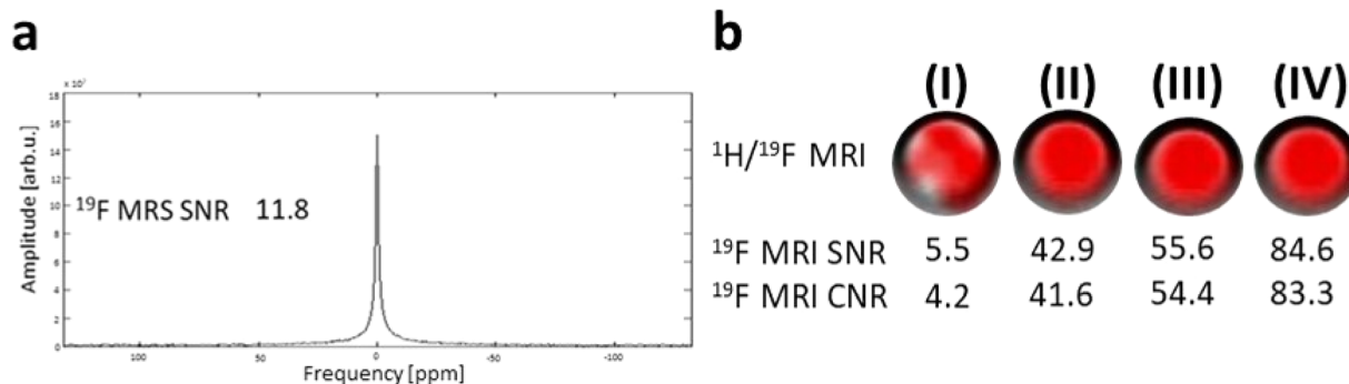
Fig. 2 Results of phantoms' ( c_{\text{pol}} = 70 \text{ mg mL}^{-1} ) ^{19}\text{F} MR signal measured on 4.7 T scanner. (a) ^{19}\text{F} MR spectrum of the polymer measured with 64 acquisitions ( \text{TA} = 1 \text{ min } 8 \text{ s} ) with given SNR and with fluorine signal peak at 0 ppm; (b) overlaid ^1\text{H}/^{19}\text{F} MRI (red – ^{19}\text{F} signal) with given ^{19}\text{F} SNR and CNR for \text{TA} = 4 \text{ s} (I) – 17 min 4 s (IV).
