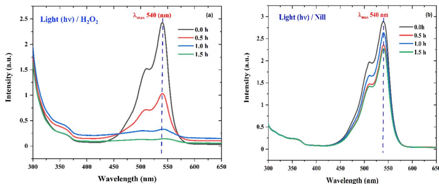
Fig. 15 (a) The UV absorption degradation curves of RhB dye with Zn-AC catalyst suspension system for the hydrogen peroxide (H 2 O 2 ) experiment in the presence of light (hv). (b) The UV absorption degradation curve of RhB dye with Zn-AC catalyst suspension system for hydrogen peroxide (H 2 O 2 ) control experiment (without H 2 O 2 in the presence of light (hv)).
