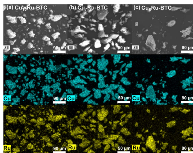
Fig. 2 SEM images (first row) and EDX elemental mapping for Cu (second row) and Ru (third row) for (a) \text{Cu}_{10}\text{Ru-BTC} , (b) \text{Cu}_7\text{Ru-BTC} and (c) \text{Cu}_6\text{Ru-BTC} . Further SEM images and the SEM-EDX spectra are displayed in Fig. S2 to S6†.
