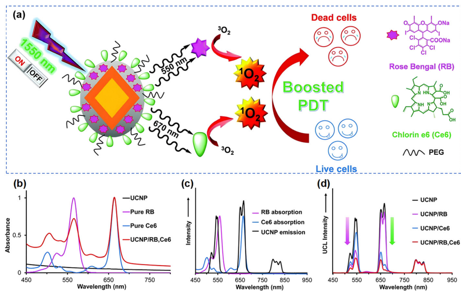
Fig. 8 (a) Schematic diagram of the formation of \text{UCNP}@(\text{SiO}_2/\text{RB/Ce6}) . (b) The absorbance of UCNPs, RB, Ce6, UCNPs/RB/Ce6. (c) The absorption and emission spectra of RB, Ce6 and UCNPs respectively. (d) The UCL spectra of UCNPs, UCNPs/RB, UCNPs/Ce6 and UCNPs/RB/Ce6 under irradiation at 1550 nm. Reproduced with permission from ref. 58. Copyright 2014, The Royal Society of Chemistry.
