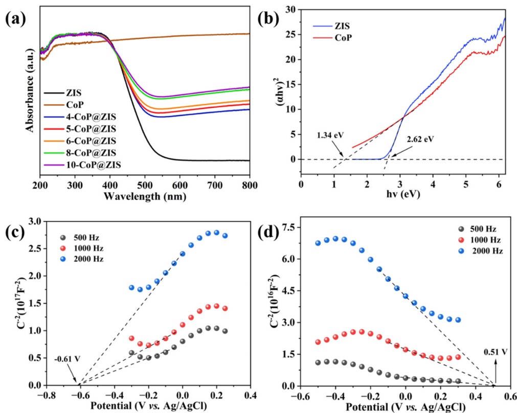
Fig. 7 (a) UV-vis diffuse reflectance spectra, and (b) the corresponding Tauc plots of different samples. Mott-Schottky plots of (c) ZIS and (d) CoP.
