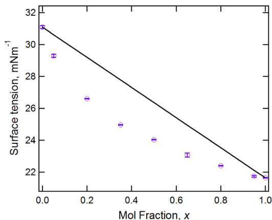
Fig. 4 Surface tension data for the mixture series [\text{C}_{10}\text{MIM}]_{1-x}[\text{C}_8\text{MIM-F}_{13}]_x[\text{TF}_2\text{N}] recorded at 20 °C.
