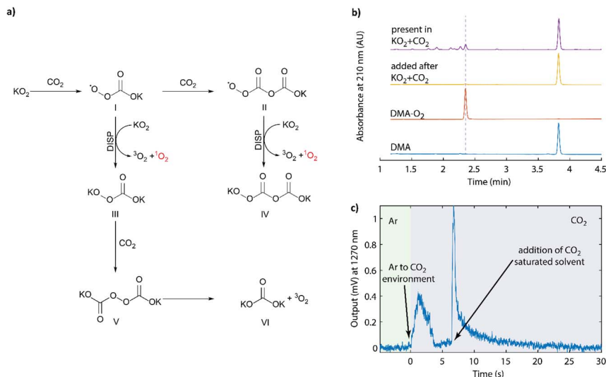
Fig. 4 (a) Reaction sequence upon reacting superoxide with \text{CO}_2 as initially described by Sawyer. 64 The final DISP step forming \text{O}_2 was identified in this work. (b) HPLC elugram of DMA exposed to asymmetric \text{K}_2\text{C}_2\text{O}_6 (yellow trace) and DMA present during the reaction of \text{KO}_2 and \text{CO}_2 (purple trace). (c) NIR output signal around 1270 nm during the reaction of \text{KO}_2 with \text{CO}_2 . The \text{KO}_2 and 50 mM 18-crown-6 suspension in \text{CH}_3\text{CN} was initially kept under Ar, then the headspace was purged by \text{CO}_2 , and then \text{CO}_2 -saturated \text{CH}_3\text{CN} was added.
