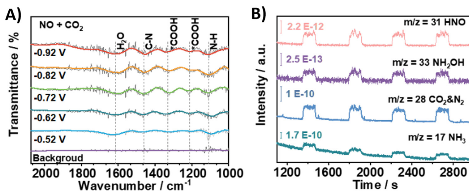
Fig. 19 Mechanistic investigations involving the formation of ^*H_2NCO using the Zn NBs catalyst. (A) In situ ATR-FTIR spectra at different potentials with NO + CO_2 as the feed gas. (B) Online DEMS measurements. Adapted from ref. 200.
