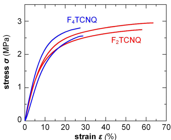
Fig. 13 Stress–strain curves measured by tensile deformation of free-standing p(g_42T-T) films co-processed with 3 mol% F_4\text{TCNQ} or 6 mol% F_2\text{TCNQ} , resulting in a similar oxidation level of 5.7 and 6.4%, respectively; Figure adapted with permission from ref. 39; Copyright 2022 (CC-BY), The Royal Society of Chemistry.
