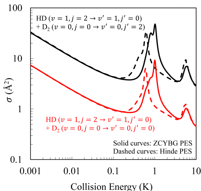
Fig. 9 Integral cross sections as a function of the collision energy for rotational quenching of HD from j_{\text{HD}} = 2 \rightarrow j'_{\text{HD}} = 0 with and without rotational excitation of the D 2 molecule from j_{\text{D}_2} = 0 to j'_{\text{D}_2} = 2 . The red curves represent the elastic transition in D 2 ( \Delta j_{\text{D}_2} = 0 ) (cross sections depicted in Fig. 5) while the black curves denote the D 2 rotational excitation channel. The solid and dashed curves show results computed on the ZCYBG and Hinde PES, respectively.
