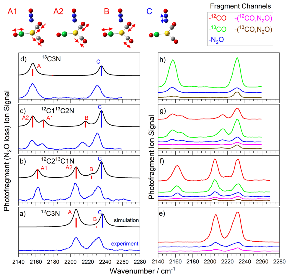
Fig. 3 (a)–(d) Comparison of experimental and simulated infrared action spectra of Au(13/12CO)3(N2O)+ complexes, recorded in the N2O loss channel. (e)–(h) Spectra recorded in different dissociation product channels, colour coded as above. For (a) and (d) A1 and A2 are degenerate and are labelled as simply A. Representations of the molecular motion in 12C213C1N is given above, here the green atom represents the 13C atom.
