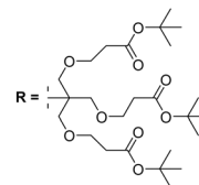
Fig. 28 General structure of the XB macrocycle series ( 52–54 ) reported by Beer et al.
