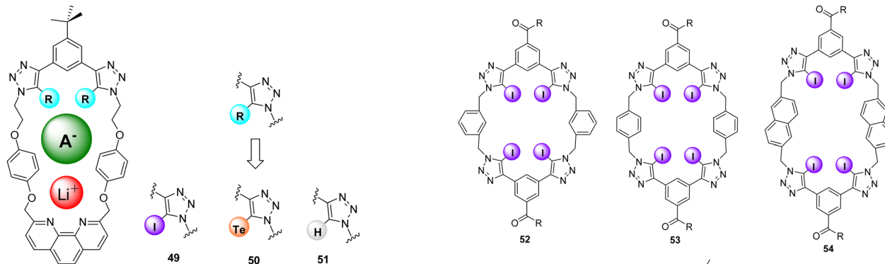
Fig. 27 Chemical structures of phenanthroline-based heteroditopic macrocycles 49 , 50 , and 51 , reported by Beer et al.
