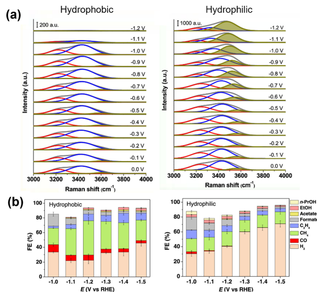
Fig. 8 (a) In situ Raman spectra of the O–H stretching mode of interfacial water molecules with hydrophobic and without (hydrophilic) modification with 1-octadecanethiol. Peaks are deconvoluted. (b) Effect of modification on \text{CO}_2\text{RR} selectivity. Reproduced with permission from ref. 68. Copyright 2021 American Chemical Society.
