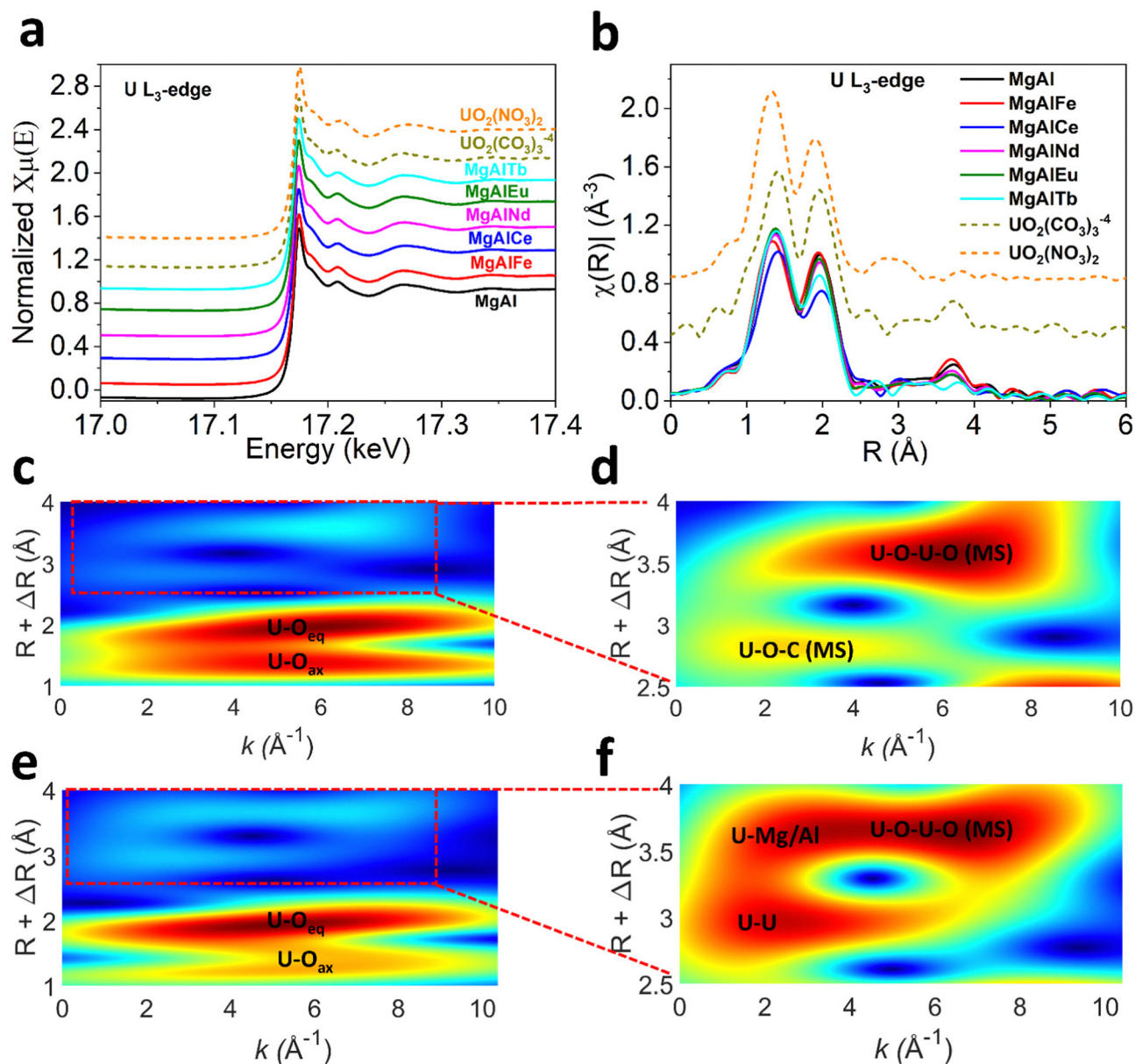
Fig. 5 U L 3 -edge XAS (a) XANES spectra (b) Fourier transformed radial plot. (c) Full-range WT representation of the EXAFS signal for UO_2CO_3 standard (1–4 Å and k_2 = 0 –10) (d) Magnified high-R WT region for UO_2CO_3 standard (2.5–4 Å and k_2 = 0 –10) (e) full-range WT for MgAl (1–4 Å and k_2 = 0 –10) (f) Magnified high-R WT region for MgAl (2.5–4 Å and k_2 = 0 –10).
