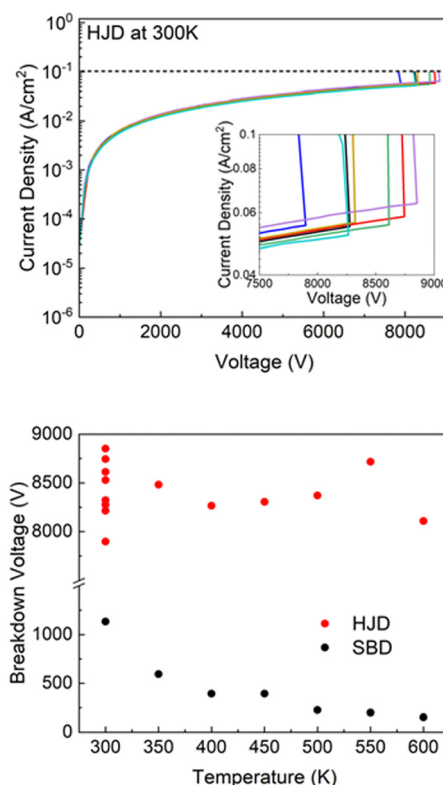
Fig. 4 (top) Spread of reverse current characteristics from \text{NiO}/\text{Ga}_2\text{O}_3 heterojunction rectifiers at 300 K. (bottom) Temperature dependence of breakdown voltage for Schottky barrier diodes and heterojunction diodes.
