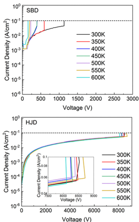
Fig. 3 (top) Reverse current characteristics from Schottky rectifiers and (bottom) \text{NiO}/\text{Ga}_2\text{O}_3 heterojunction rectifiers as a function of temperature.
