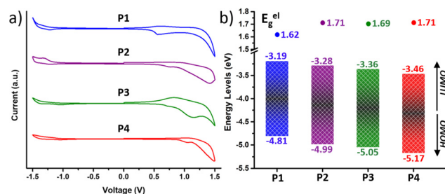
Fig. 4 (a) Cyclic voltammograms as a thin film (scan rate 100 \text{ mV s}^{-1} ) and (b) HOMO–LUMO energy levels of the copolymers P1–P4 .
