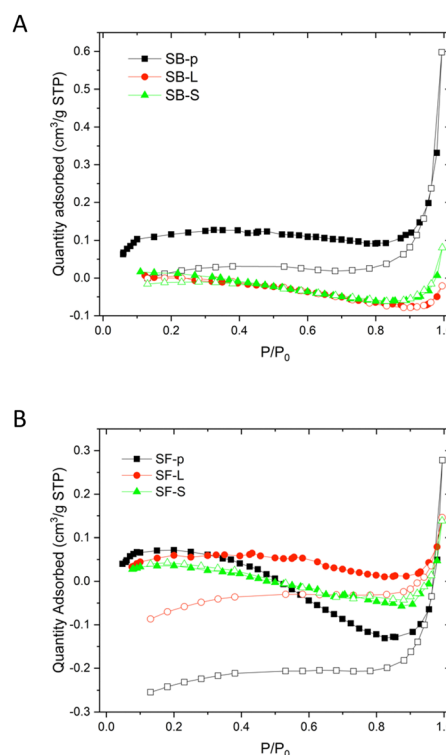
Fig. 6 Isotherms obtained from sphere derived samples showing negligible or no gas adsorption. (A) Granules derived from 3D printed sphere blocks: large (SB-L); small (SB-S); pulverized (SB-p). (B) Granules from sphere foam blocks: large (SF-L); small (SF-S); pulverized (SF-p).
