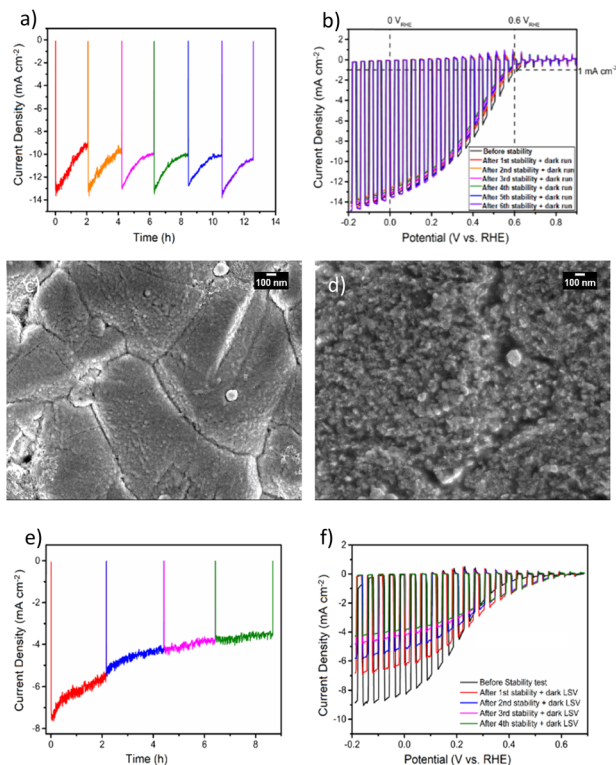
Fig. 4 (a) Current–time curve of CZTS/CdS/ITO/Pt in 1 M K 2 HPO 4 /KH 2 PO 4 (pH 7) under solar simulated AM 1.5G light irradiation at an applied bias of 0 V RHE . The stability test is conducted at 2 h intervals with 3 recovery dark LSV sweeps at every interval. (b) Corresponding chopped LSV before the stability test and after each recovery dark LSV sweep. Scanning electron microscopy (SEM) of CZTS/CdS/ITO/Pt after 12 h stability test (c) with recovery dark LSV (d) without recovery dark LSV sweeps. (e) Stability test and (f) corresponding LSV for the photocathode without ITO (CZTS/CdS/Pt).
