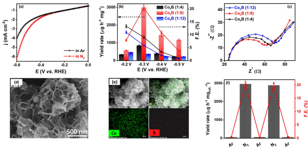
Fig. 1 (a) Linear sweep voltammograms for \text{Co}_2\text{B} (1 : 8) in \text{Ar} - and \text{N}_2 -saturated 0.1\text{ M KOH} , (b) comparison of yield rates and F.E. of \text{Co}_2\text{B} catalysts at different applied potentials, (c) Nyquist plots, (d) FE-SEM image of \text{Co}_2\text{B} (1 : 8) and (e) corresponding elemental dot mapping showing uniform distribution of Co and B elements over the scanned area. (f) F.E. and yield rates obtained during NRR under switching gas-feed ( \text{Ar}/\text{N}_2 ) environments.
