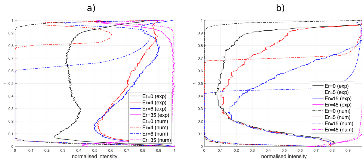
Fig. 5 Normalized light intensity (a) at a 135° angle from the U-bend entrance; (b) between the inner and outer corner of the L-bend. r denotes the normalized distance from the outer U-bend wall and from then inner corner in the L-bend, respectively.
