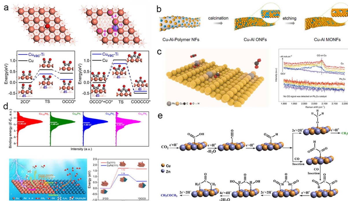
Fig. 4 (a) Adsorption energies of ^*CO at Cu and Cu_{vac}-Ti sites (above). Energy profiles for ^*CO dimerization and trimerization at the Cu and Cu_{vac}-Ti sites (below). The purple, orange, red, and gray spheres represent Ti, Cu, O, and C atoms, respectively. Reproduced from ref. 106. Copyright 2021 Wiley-VCH. (b) Schematic representation of the preparation of Cu–Al MONFs. Reproduced from ref. 107. Copyright 2022 American Chemical Society. (c) Schematic illustration of CO_2 conversion into HCOOH over a Pb_1Cu SAA (left). In situ Raman spectra recorded at different current densities for Cu and Pb_1Cu SAA catalysts, showing the absence of CO formation on the Pb_1Cu catalyst (right). OCV, open-circuit voltage. Reproduced from ref. 108. Copyright 2022 Nature. (d) Surface valence band photoemission spectra of different CuPd catalysts (above). Schematic diagram of the mechanism of the Cu–Pd catalyst for facilitating the production of C_{2+} products from ECR. Energy profile of ^*CO coupling at the Cu domain and phase-separated Cu–Pd interface (below). Reproduced from ref. 113. Copyright 2023 Wiley-VCH. (e) Possible mechanisms for producing methanol and acetone on the Cu/Zn nanoalloys. Reproduced from ref. 71. Copyright 2022 Royal Society of Chemistry.
