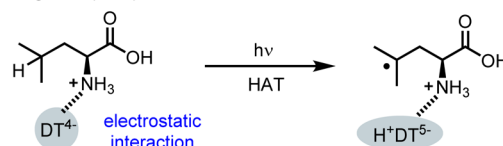
b) Proposed electrostatic interaction for accelerating C–H abstraction by decatungstate (DT⁴⁻)
