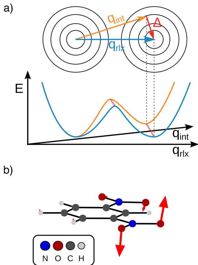
Fig. 7 (a) Schematic representation of the separable intrinsic ET coordinate (Marcus dimension, q_{\text{int}} , orange) and orthogonal structural relaxation ( \Delta , red arrow) vs. the relaxed ET coordinate ( q_{\text{rlx}} , blue) that may be obtained from a LICC approach. (b) Structural relaxation obtained by LICC between the second minimum at the Marcus dimension and fully optimized geometry.
