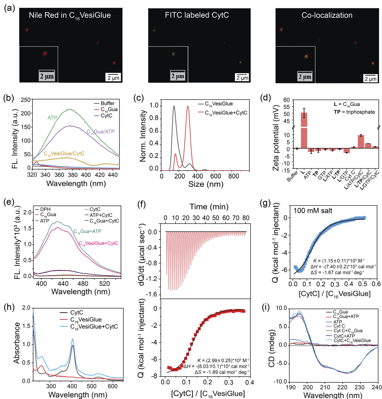
Fig. 3 VesiGlue for the molecular recognition of proteins. (a) Representative CLSM images showing Nile red stained C 16 VesiGlue (red fluorescence), FITC-labeled CytC (green fluorescence) and co-localized (orange) ATP-templated structures. (b) Fluorescence intensity of ATP (green) at λ exc. 260 nm upon interaction with C 16 Gua forming VesiGlue (purple) and CytC (yellow). (c) NTA measurements of C 16 -VesiGlue (black) with CytC glued on the surface (red). (d) Zeta potential of XTP/C 16 Gua (X = G, sodium) systems (1 : 3 molar ratio) in the presence of CytC in buffer. n = 3 technical replicates, mean ± SD for all the studies. (e) DPH dye leakage experiment. The fluorescence intensity of DPH (λ exc. 355 nm) containing assembly was measured upon CytC addition. (f) Top: Raw ITC thermogram of CytC titrated into C 16 VesiGlue in 1 mM HEPES buffer (pH 6), exhibiting exothermic peaks. Bottom: Integrated heat flow signals as a function of CytC/VesiGlue molar ratio. The best fit was obtained by a single-site non-competitive binding model, demonstrating a highly favorable binding affinity. (g) Integrated heat flow obtained from the ITC thermogram for the titration of CytC into C 16 VesiGlue in the presence of 100 mM salt concentration. (h) UV-vis spectral scan of CytC (black), VesiGlue (red) and CytC in the presence of VesiGlue (blue) shows the unaffected heme centre of CytC upon binding to VesiGlue. (i) CD spectra of CytC in the presence of VesiGlue and the appropriate controls demonstrating the stability of the secondary structure of CytC.
