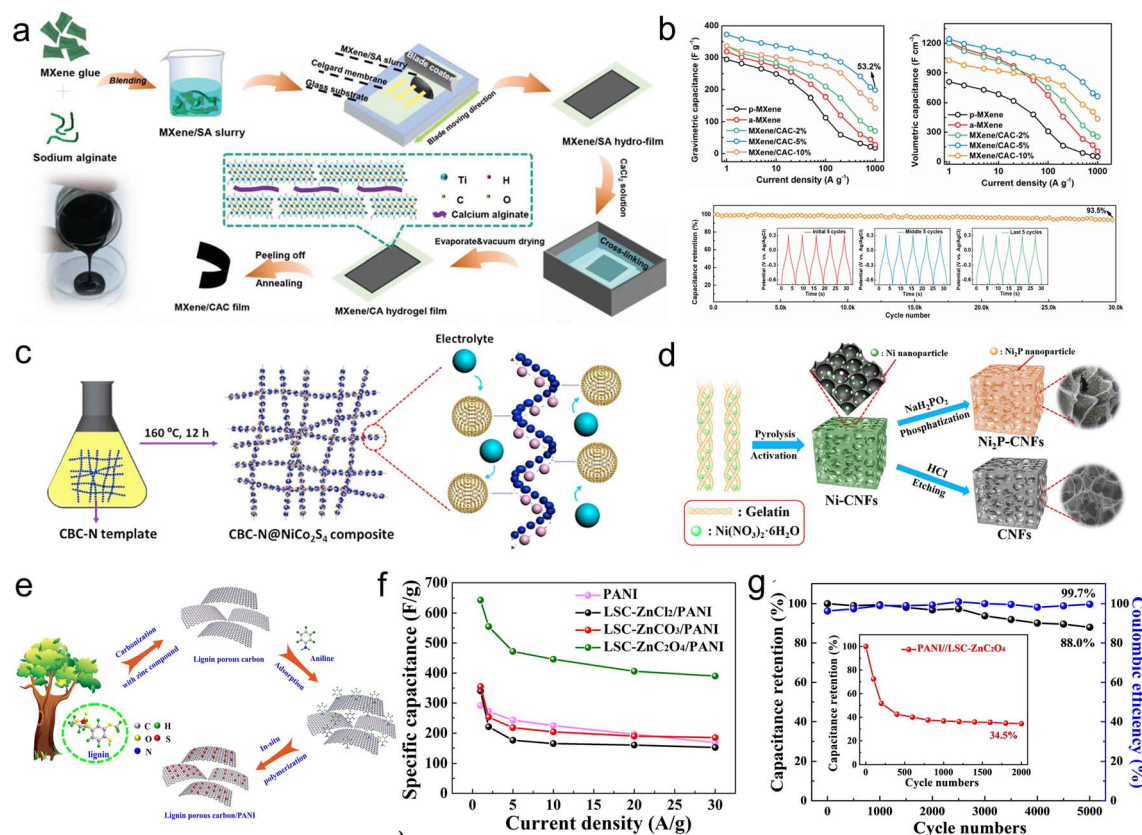
Fig. 12 (a) Scheme for the synthesis of MXene/CAC films; 150 (b) capacity and cycling stability test of MXene/CAC; 150 (c) scheme for the space-confined growth of CBC-N@NiCo 2 S 4 composite; 155 (d) diagrams for the preparation of Ni-CNFs, Ni 2 P-CNFs and CNFs; 156 (e) schematic for the fabrication of lignin porous carbon/PANI composites; (f) specific capacitance of the samples; (g) cycling test of LSC-ZnCo 2 O 4 /PANI//LSC-ZnCo 2 O 4 ASCs. 161
