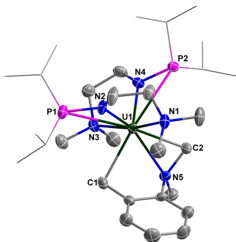
Fig. 5 Molecular structure of 4 with thermal ellipsoids at the 50% probability level. Hydrogen atoms are omitted for clarity. The i Pr groups on P atoms are simplified into lines. Selected bond distances (Å): U1–N1 2.734(4), U1–N2 2.297(3), U1–N3 2.813(4), U1–N4 2.285(4), U1–N5 2.568(3), U1–P1 3.2145(11), U1–P2 3.1286(11), U1–C1 2.553(4), U1–C2 2.461(4).
