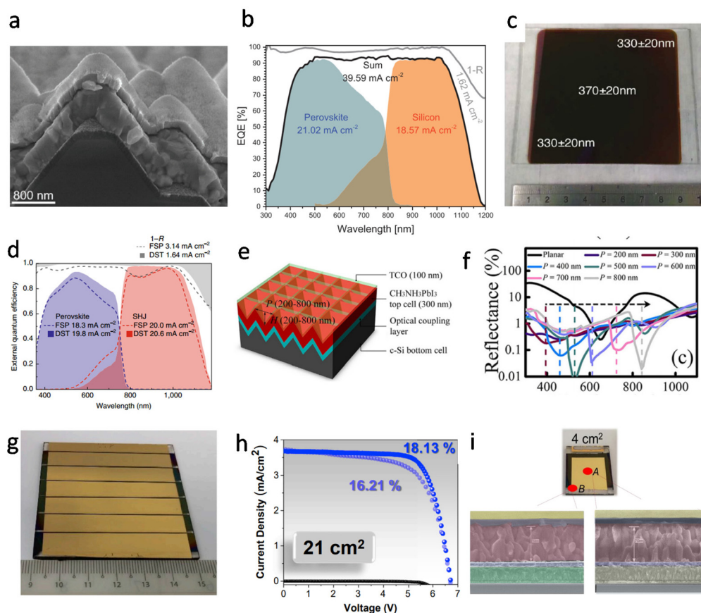
Fig. 9 (a) Cross-sectional SEM image of textured silicon bottom cells covered with MA 0.5 FA 0.63 PbI 3.13 , capped with 18 nm of C 60 and after the 20 nm SnO 2 ALD deposition. Reproduced with permission. 110 Copyright 2021, Wiley-VCH. (b) EQE and reflection spectra (denoted as 1 - R) including the integrated current densities of the two sub cells, the sum and reflection. Reproduced with permission. 110 Copyright 2021, Wiley-VCH. (c) Photograph of 8 cm × 8 cm thin film of FAPbI 3 deposited on a glass substrate. The image shows the substrate after thermal annealing at 170 °C for 1 min. The results of thickness measurements at three positions are superimposed on the image, and a metal ruler with a centimeter scale is shown as a size reference. Reproduced with permission. 116 Copyright 2017, American Chemical Society. (d) Improved optics with a fully textured architecture. EQE of perovskite/SHJ monolithic tandem cells with double-side-textured (DST) or front-side-polished (FSP) bottom cells, alongside corresponding total absorbance curves, 1 - R, where R is the reflectance of the device. These EQE and 1 - R spectra do not include losses due to the front-side metal grid. Reproduced with permission. 113 Copyright 2018, Springer Nature. (e) Schematic of perovskite/c-Si tandem solar cells (TSC) with inverted nanopillar structure. The parameters H and P denote the pyramid height and its period, respectively. (f) Reflectance of inverted nanopillar perovskite/c-Si TSC. Reproduced with permission. 115 Copyright 2015, Springer Nature. (g) Image of a 21 cm 2 active area perovskite solar module consisting of 6 series-connected sub-cells. Reproduced with permission. 54 Copyright 2020, Elsevier Inc. (h) Treated-MAPbI 3 perovskite solar module dark, forward, and backward J-V curves measured in air. Reproduced with permission. 54 Copyright 2020, Elsevier Inc. (i) 4 cm 2 PSC photograph and cross-sectional SEM images of point A and point B. Reproduced with permission. 54 Copyright 2020, Elsevier Inc.
