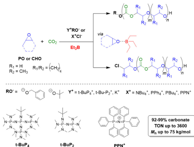
Scheme 1 The first metal-free copolymerization of epoxides and \text{CO}_2 , enabled by \text{Et}_3\text{B} as epoxide activator. Note that initiation can be achieved via alkoxides or chloride.
