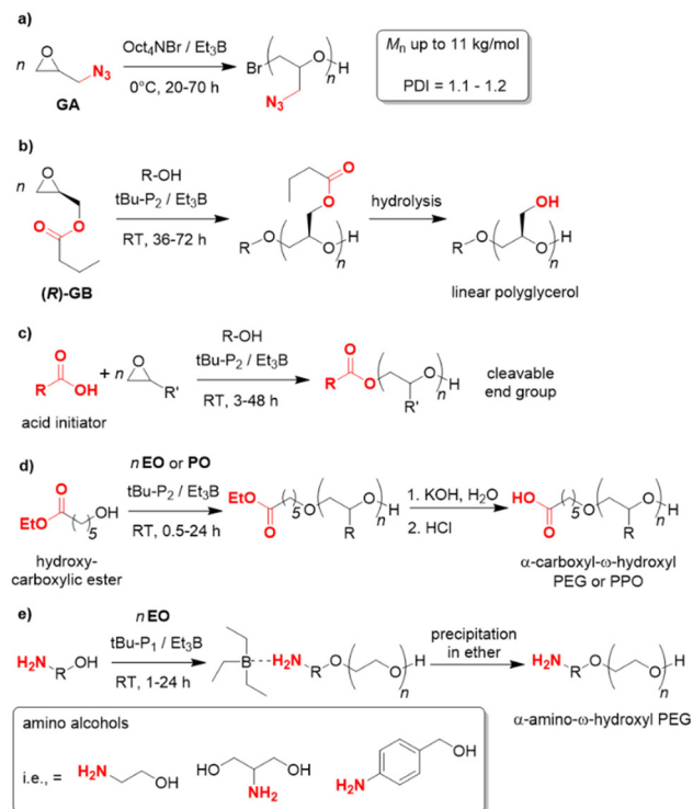
Scheme 9 Functional group tolerance as a distinctive feature of Et 3 B-mediated polymerization catalysis.
