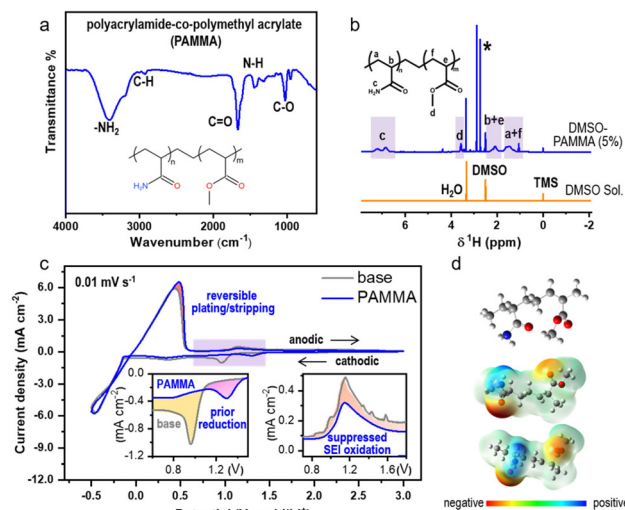
Fig. 1 (a) FTIR and (b) ^1\text{H} -NMR characterization of the PAMMA molecule; structure formulas are exhibited as insets. (c) CV curves in \text{O}_2 atmosphere without (gray trace, 1.0 M LiTFSI in TEGDME)/with (blue trace) PAMMA addition. Scan rate: 0.01 \text{mV s}^{-1} ; potential range: -0.5 – 3.0 V. The insets in the left and right represent partial enlarged cathodic and anodic peaks without and with PAMMA, respectively. (d) ESP calculation of the PAMMA molecule by Gaussian09 with different views. The ball-and-stick model of PAMMA is embedded.
