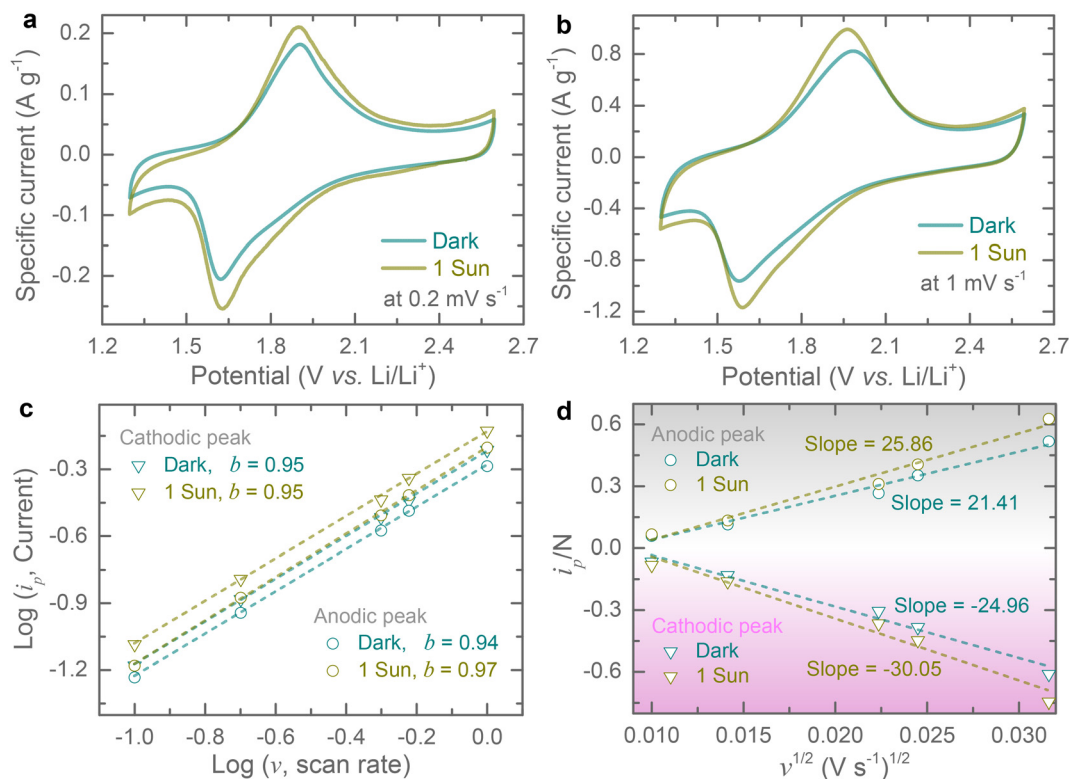
Fig. 3 Electrochemical performance of Cu-HHB electrodes both in the dark and 1 sun illumination. (a and b) CV profiles at 0.2 mV s -1 and 1 mV s -1 in the dark and 1 sun illumination. (c) Plots of log( i p ) vs. log( v ): estimation of b -values for cathodic and anodic peaks in the dark and 1 sun illumination. (d) Estimation of Li-ion diffusion constant improvements under illumination from i p / N vs. v 1/2 curves.
