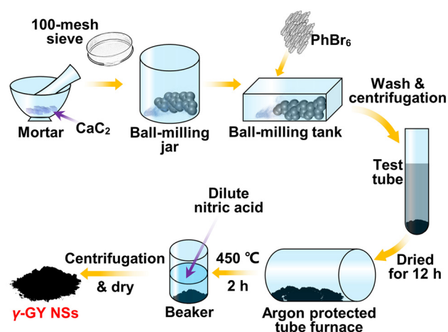
Fig. 1 Preparation flow chart of \gamma -GY NSs.
