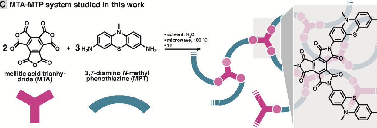
Scheme 1 Polyimide syntheses. (A) Classical polyimide (PI) synthesis from anhydride and amine co-monomers via polyamic acids (isolable). (B) Hydrothermal PI synthesis from anhydride and amine monomers via ammonium carboxylate monomer salts (MS). (B) Typical reaction conditions indicated on arrows. * designates non-specified end-group. (C) Hydrothermal synthesis and designated structure of mellitic trianhydride (MTA) and 3,7-diamino-N-methylphenothiazine (MPT)-based PI network systems used in this study. Network schematic: MTA in red, MPT in blue, imide linkages in light red.
