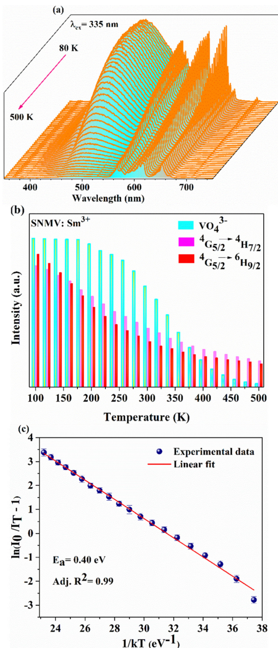
Fig. 5 (a) Temperature-dependent PL spectra of \text{Sr}_2\text{NaMg}_2\text{V}_3\text{O}_{12}:0.05\text{Sm}^{3+} under 335 nm excitation, (b) the histogram showing the relative reduction in the intensity of dual emission from (\text{VO}_4)^{3-} and \text{Sm}^{3+} ions, and (c) linear fit of the Arrhenius equation.
