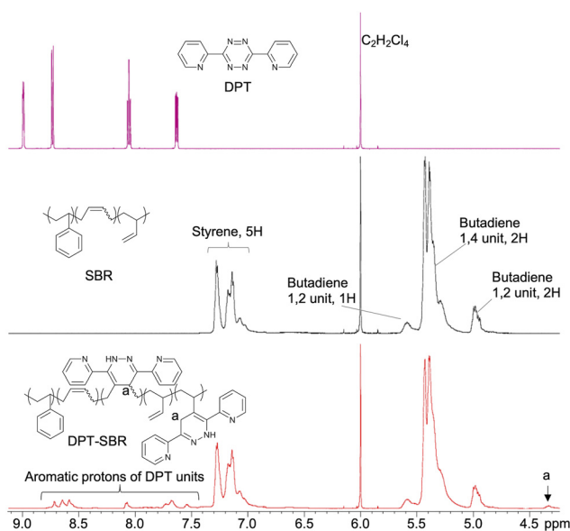
Fig. 4 1 H NMR spectra of DPT, SBR and DPT-SBR3.
