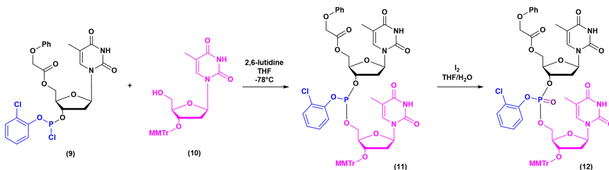
Fig. 5 Phosphotriester method by Letsinger, applied to the synthesis of dithymidynyl nucleotide (12) (1976).
