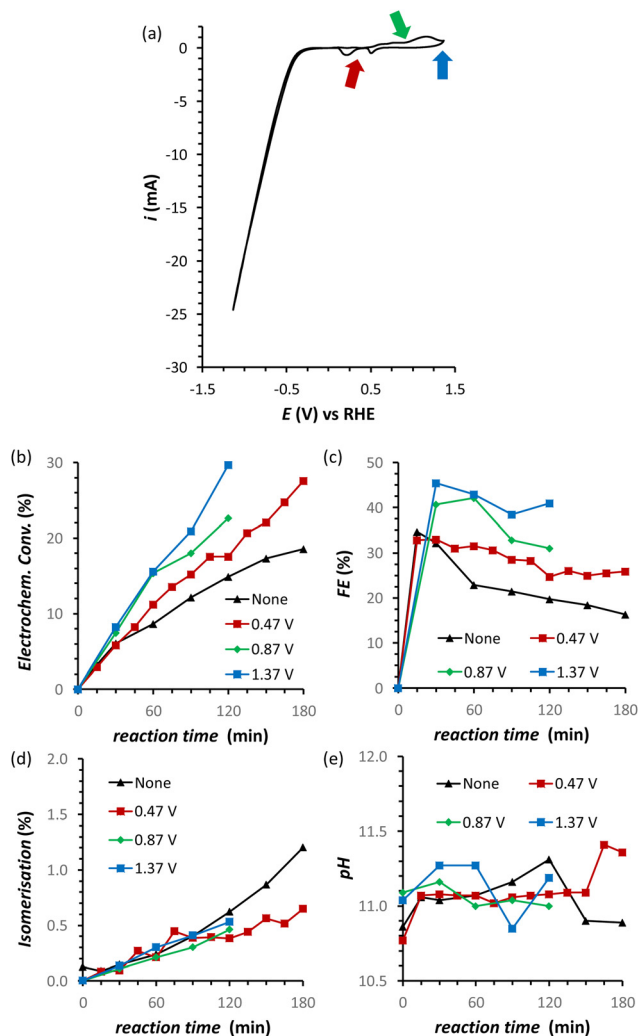
Fig. 6 (a) Cyclic Voltammetry (CV) of the Cu-wire electrode at 50 mV s^{-1} scan rate sweeping in a potential window from 1.37 V to -1.3 V vs. RHE. (b–d) Effect of oxidative pulses on the FRR on a Cu-wire electrode in a 0.12 M PBS solution at pH_{initial} = 11.3 : (b) electrochemical conversion, (c) Faradaic efficiency, (d) isomerisation and (e) the pH. Conditions: i = -20 mA ( j = -5.3 mA cm^{-2} ), AMVN membrane as separator, constant pH titration with 10 \mu L min^{-1} of 0.5 M H_3PO_4 , 3 h at room temperature (21 ^{\circ}C ).
