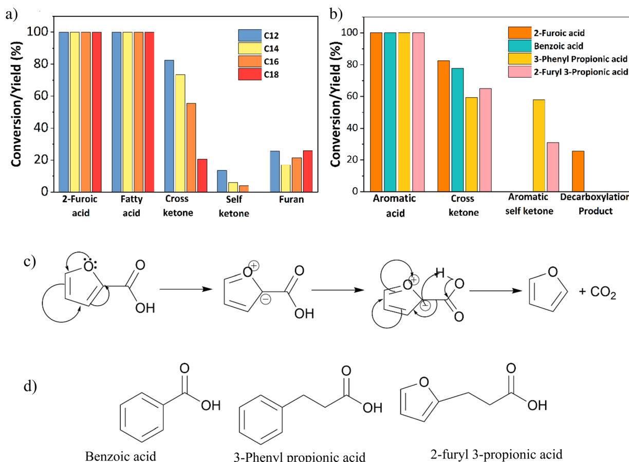
Fig. 5 Effects of fatty acid chain length and aromatic acid structure (a) 0.25 M 2-furoic acid, 0.15 M fatty acid, 30 ml dodecane, 350 °C, 90 min, 20 bar \text{N}_2 , 800 rpm, 0.2 g MgO catalyst. Impact of different ring chemistry (benzoic acid) and aromatic acids with \alpha -hydrogens (2-furyl propionic acid, 3-phenyl propionic acid). (b) 0.25 M aromatic acid, 0.15 M lauric acid, 30 ml dodecane, 350 °C, 90 min, 20 bar \text{N}_2 , 800 rpm, 0.2 g MgO catalyst. (c) A decarboxylation mechanism for 2-furoic acid is reported in the literature. 35 (d) Structures of the different aromatic acids tested.
