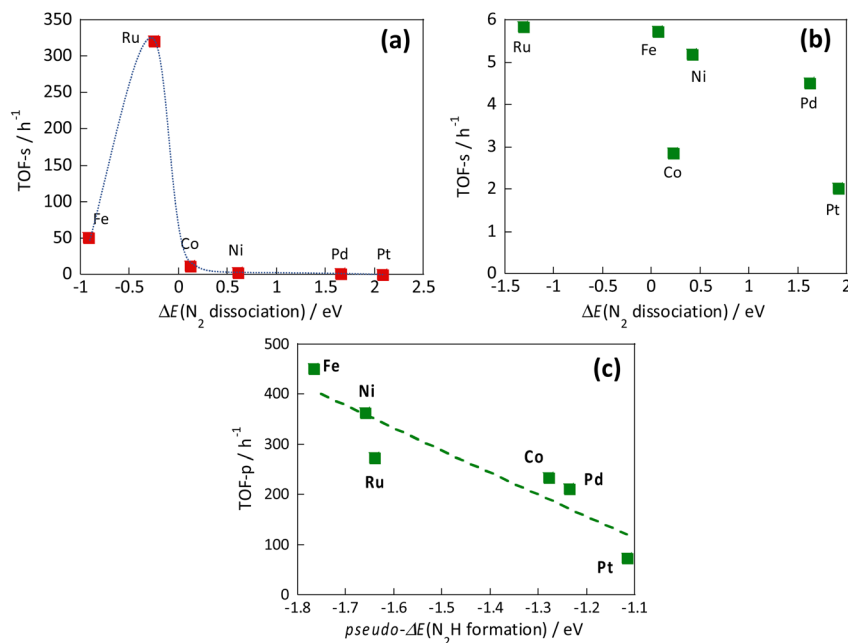
Fig. 13 Correlation between the N_2 dissociation energy and the TOF-s of the catalytic reaction upon heating (a), correlation when the electric field is applied (b), and correlation between N_2H formation energy and TOF-p (c). 36
